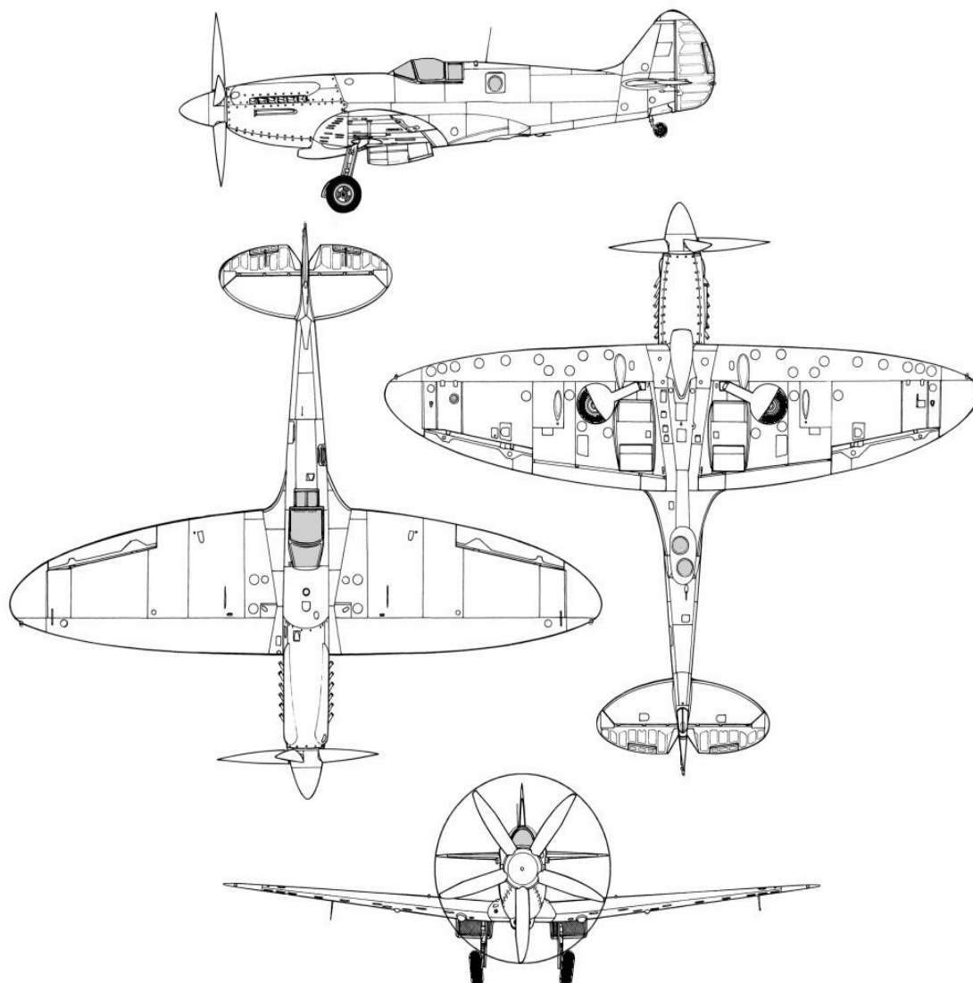
Supermarine Spitfire PR-XI
