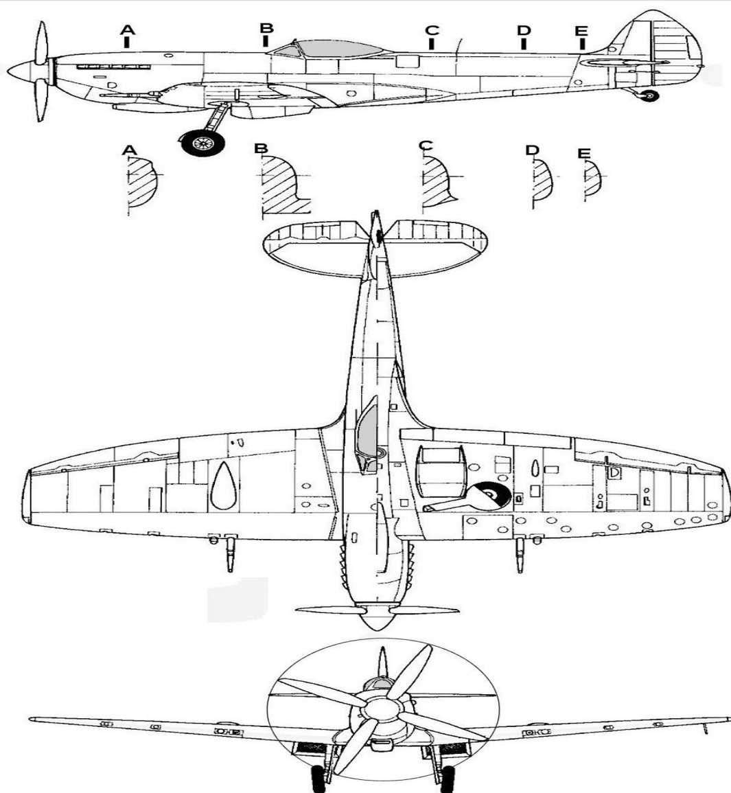
Supermarine Spitfire Mk XVI LF
