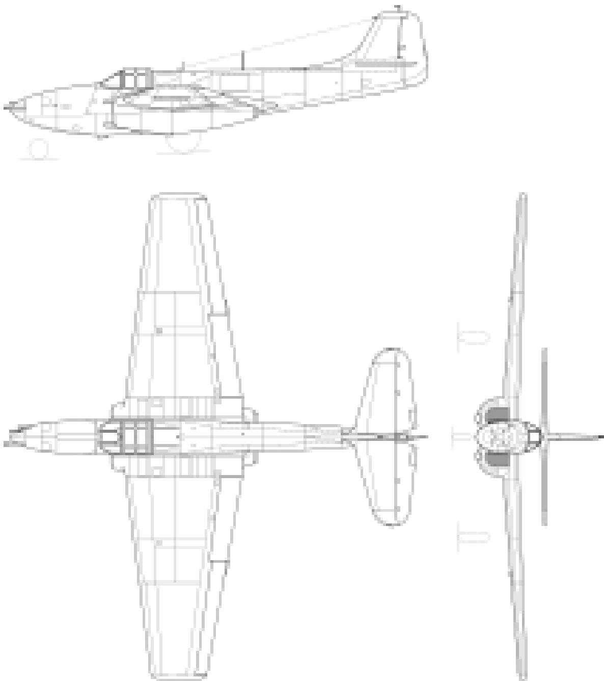
3-view drawing of the P-59
