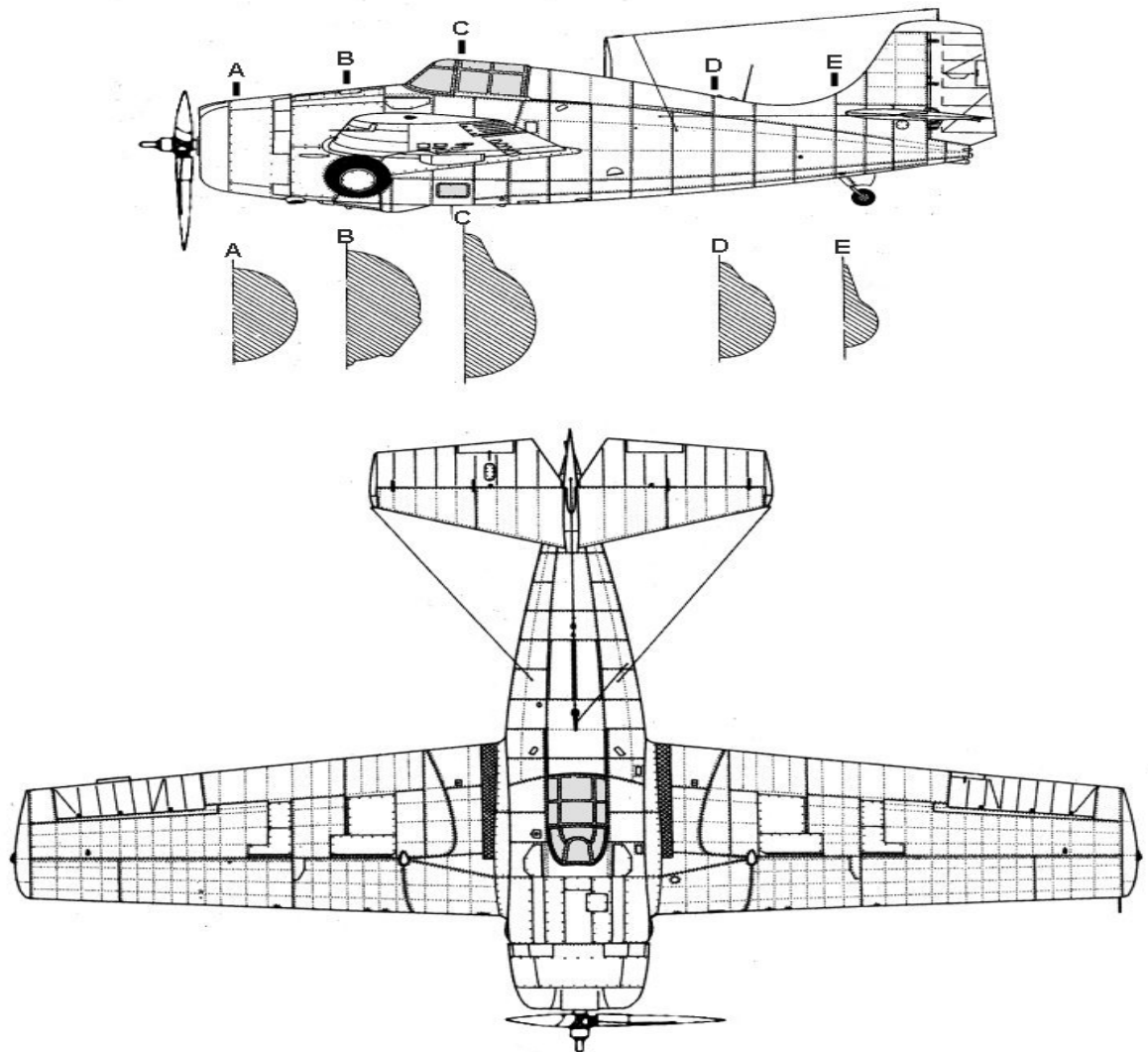
Grumman F-4F4 Wildcat
